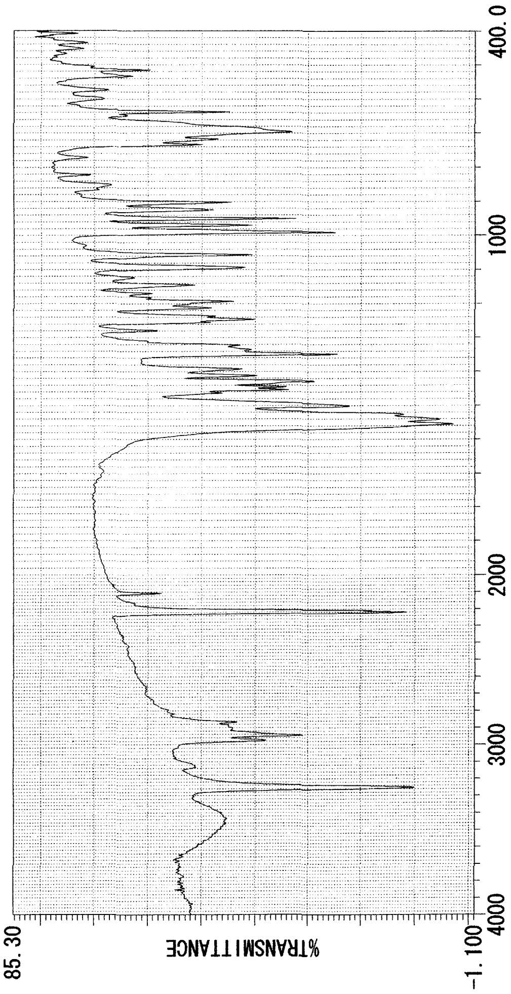
Wavenumbers (cm -1 )
