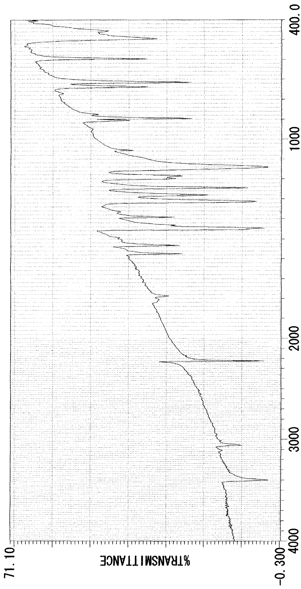
Wavenumbers (cm -1 )
