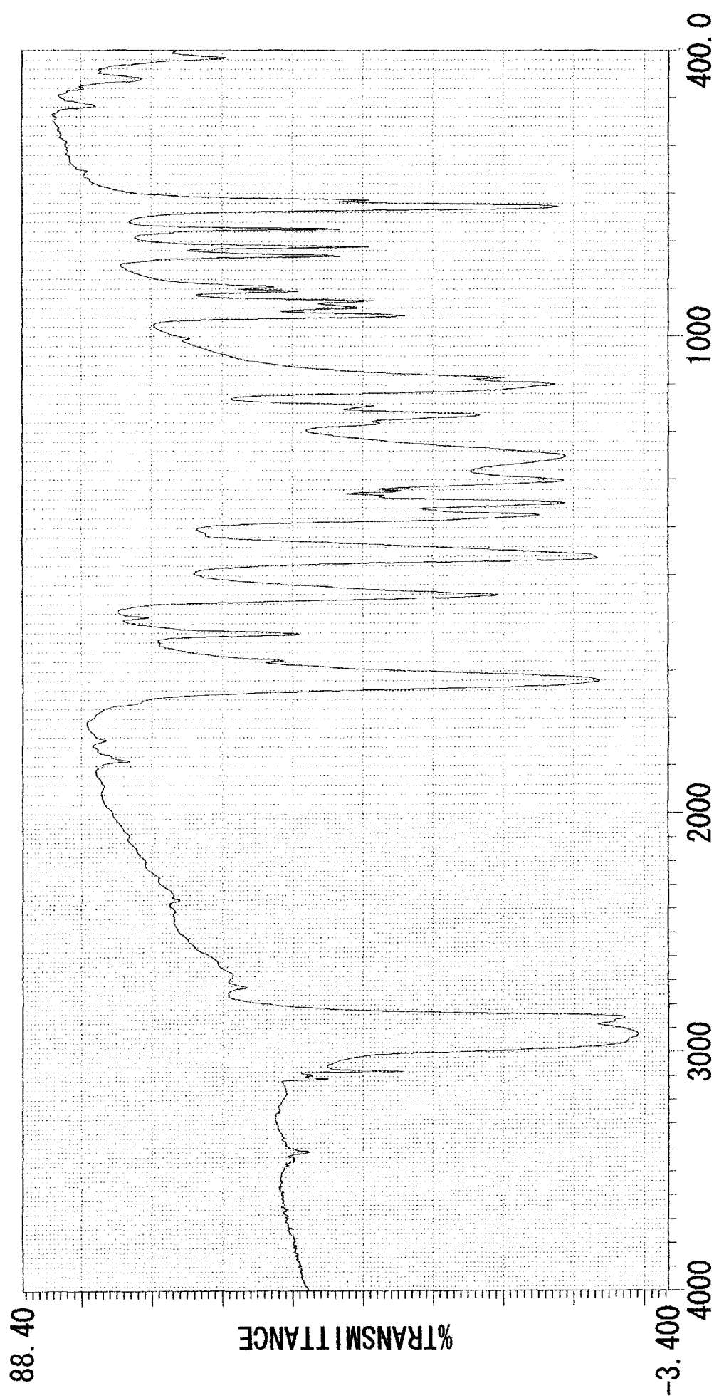
Wavenumbers (cm -1 )
