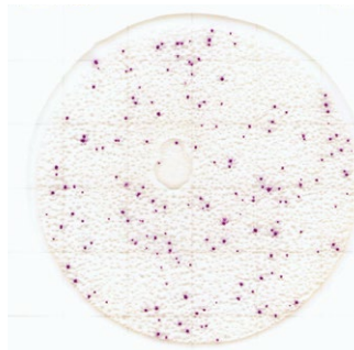
Zygosaccharomyces rouxii
