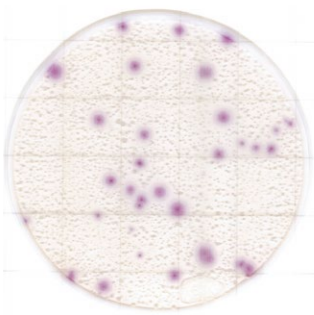
Aureobasidium pullulans
