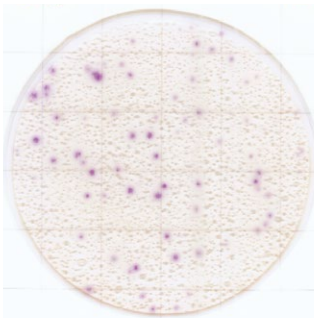
Penicillium glabrum
